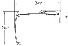
Smooth Face
