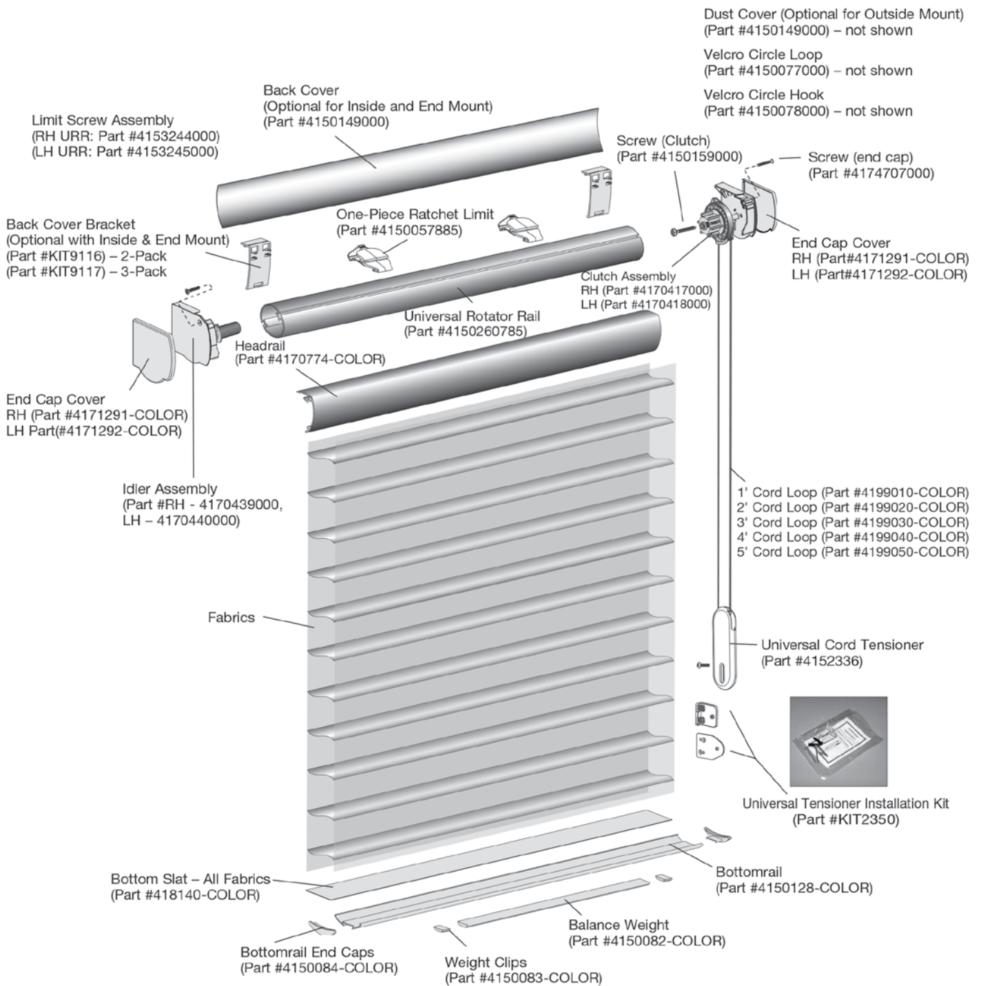
BACK COVER BRACKET (Part #KIT9116) – 2-Pack (Part #KIT9117) – 3-Pack
